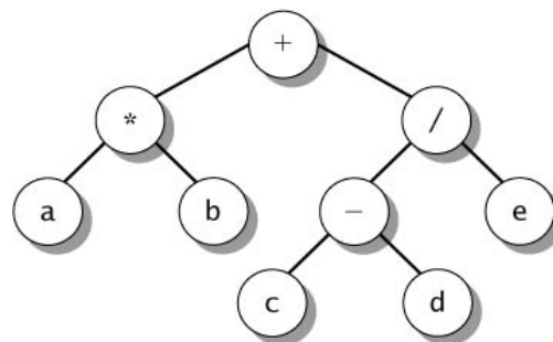
Gambar 8. Binary Tree Studi Kasus 2
