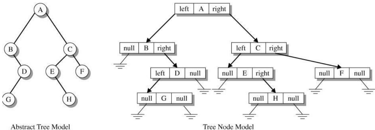
Abstract and tree node model of a binary tree.
