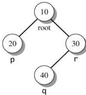
Gambar 6. Contoh Binary Tree
